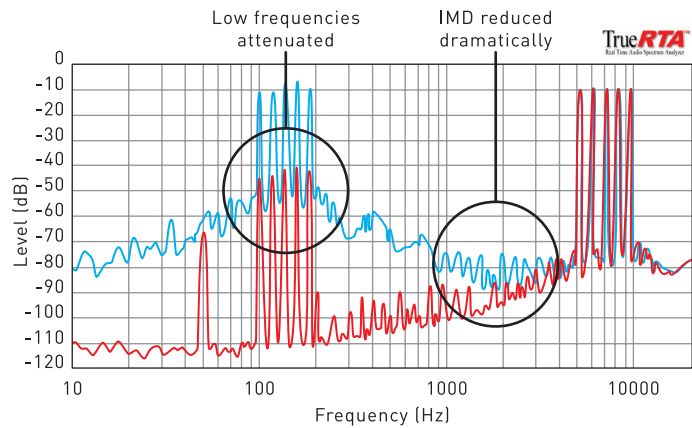
Figure 28. Spectral analysis of the output of a current probe measuring cable current in the tweeter cable of a biwire connection (red trace), overlaid on the single-wire trace from Figure 27
