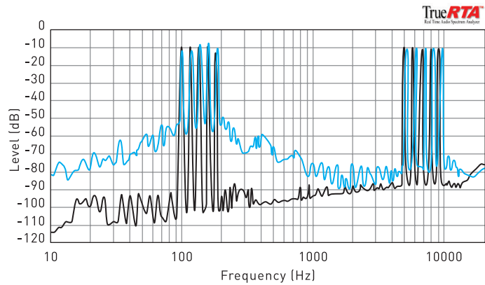
Figure 27. Spectral analysis of the output of a current probe measuring cable current in the single-wire connection (blue trace), overlaid on the trace from Figure 26
